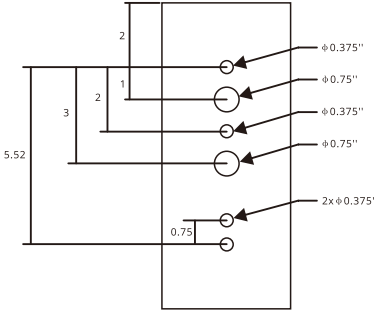
LumESCO Universal LumCADEN/LumPLEX Pole Drill Pattern All units in inches
