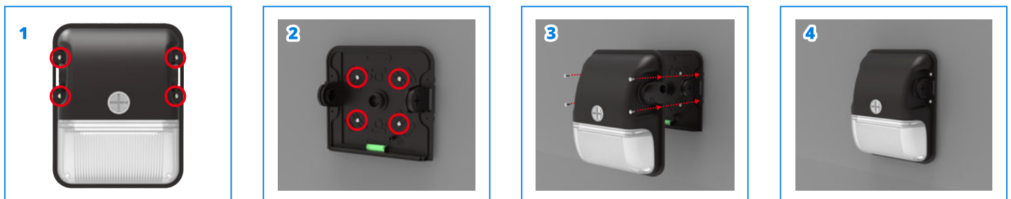
Fig.1: Remove four side screws of luminaire.
