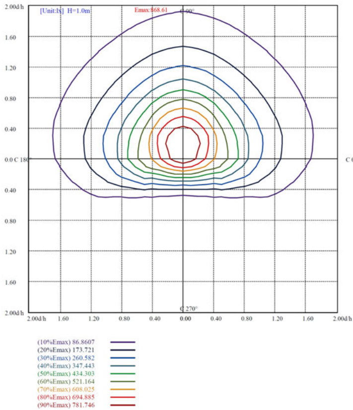
ISO illuminance diagram(Lux) of 3000K
