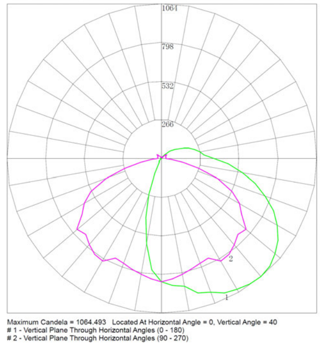
Polar Curves of 3000K
